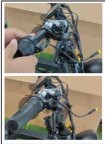
22. Install throttle and short handle sleeve
