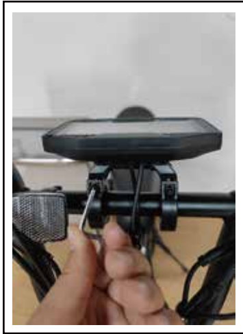
19. Install the dashboard and tighten all screws
