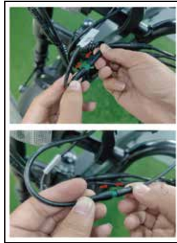
20. Connect the ports of cables according to the direction of arrow
